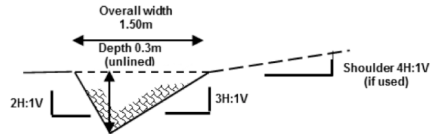
Figure 6 Example of a drain width design
