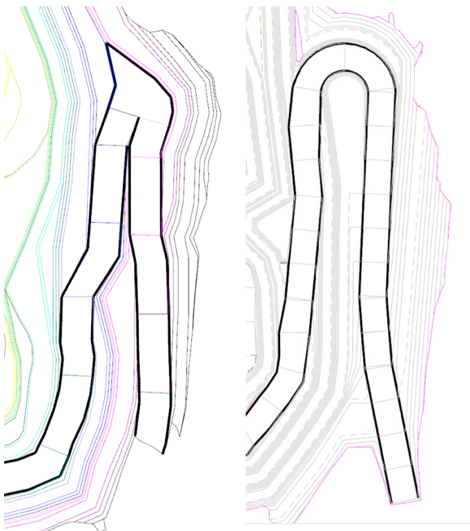
Figure 10 Example of a vertical curve change at ramp gradient change to maintain line of sight
