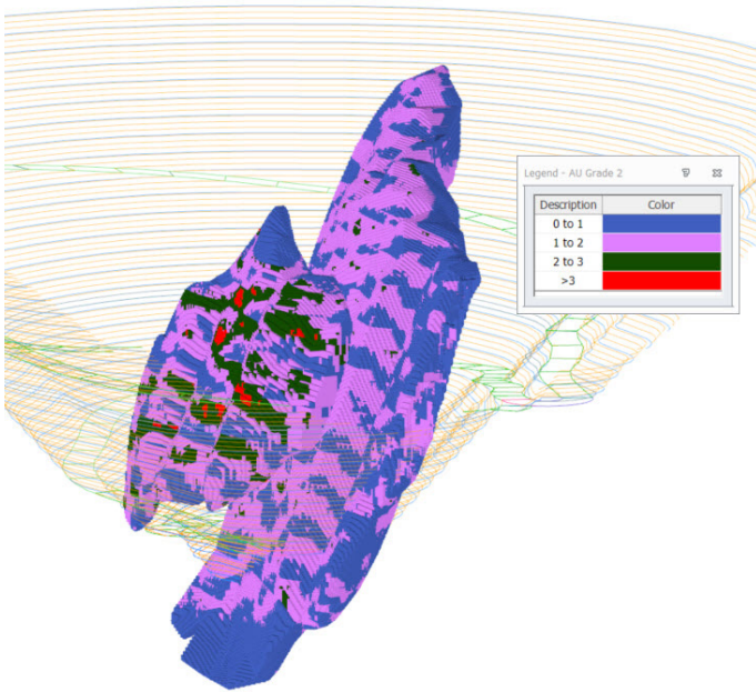
Figure 1: A block model of an ore body coloured by grade (shell and slice)
