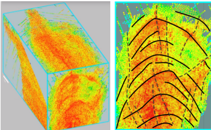
Figure 30: Example of how structure can be interpreted with grade samples plotted on projection to symmetry plane
