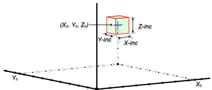
Figure 3: Block model block definition
