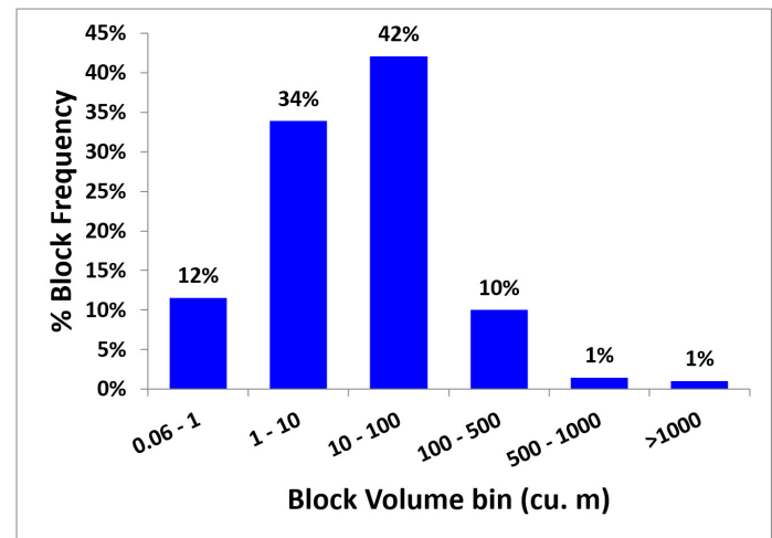
Figure 32: Distribution of size of ore lode blocks by number frequency and volume in the unregularized sub-celled model
