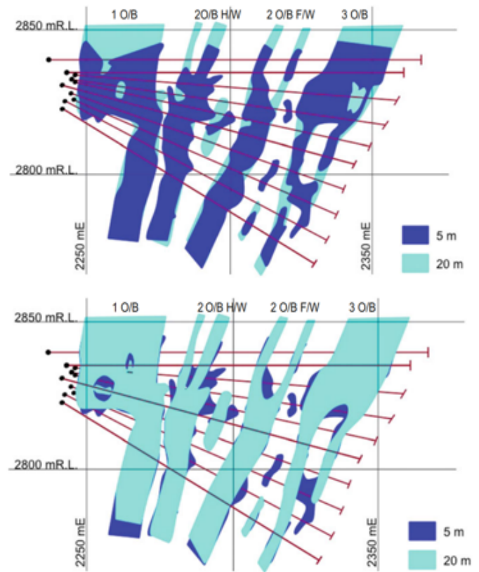
Figure 23: Cross-sectional interpretation based on 20m and then 5m drill spacing
