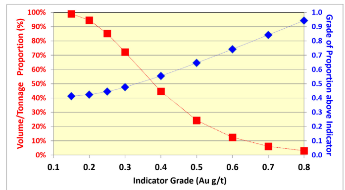
Figure 16: Example of MIK model tonnage-grade distribution for a single block
