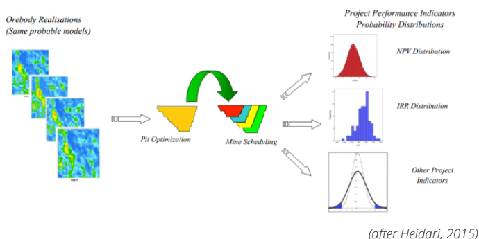
Figure 19: Risk-based method for mine planning using ConSim
