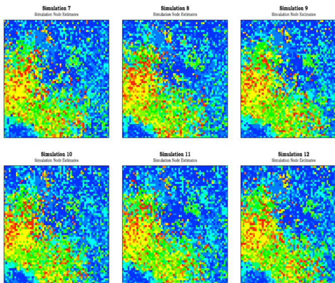
Figure 19: Risk-based method for mine planning using ConSim
