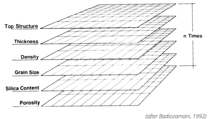
Figure 20: Structure of a gridded seam model
