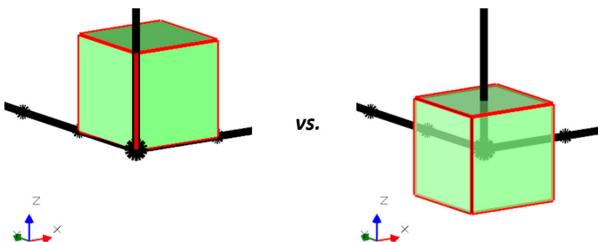
Figure 5: Potential block centroid to origin relationship
