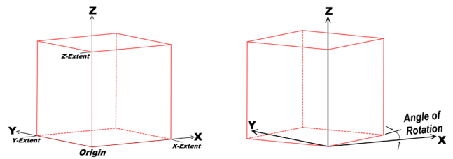
Figure 2: Standard block model framework
