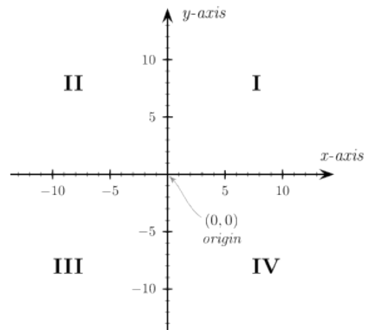
Figure 13: Cartesian quadrants
