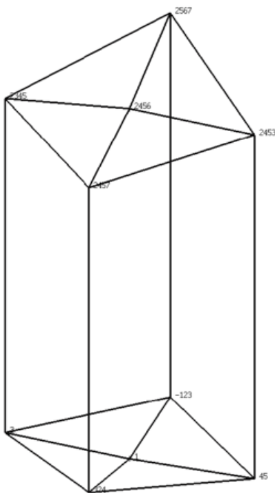
Figure 21: Diagrammatic view of single HARP block, showing corner relative levels
