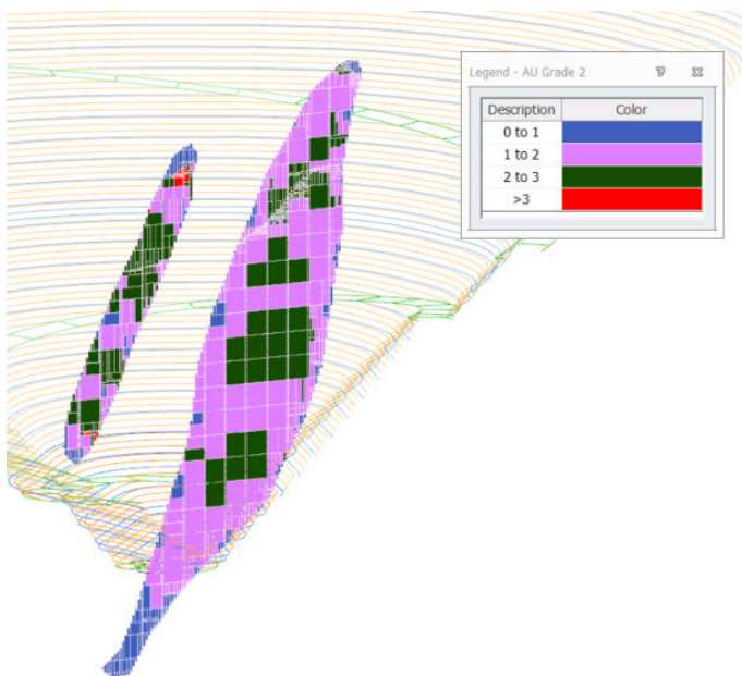
Figure 3: Block model block definition
