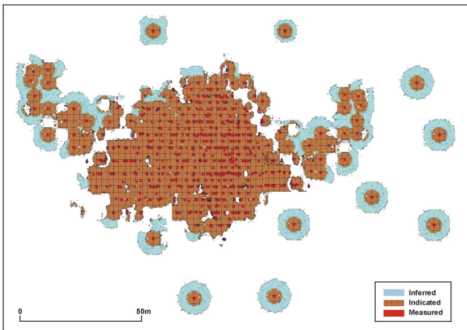
Figure 28: The “spotted dog” geological model
