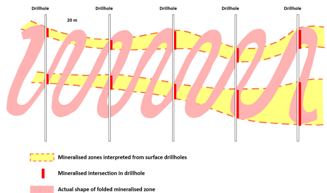
Figure 26: Interpretation versus actual ore structure at Stekenjokk mine
